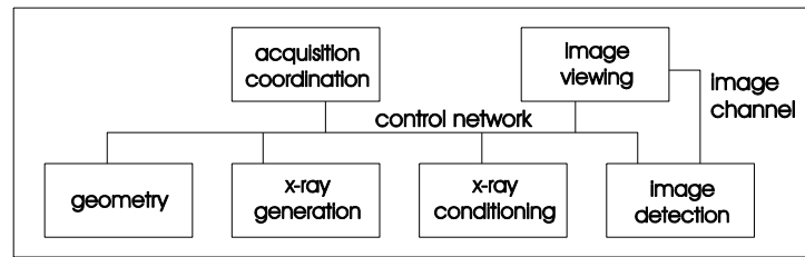
Figure 6. Technology architecture
