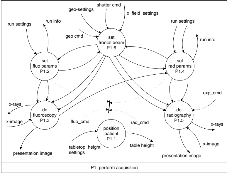
Figure 4. Functional architecture
